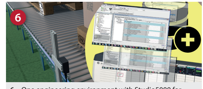
6. One engineering environment with Studio5000 for configuring and programming of all facets: Logix, HMI, Stratix 5700, PowerFlex, Kinetix, MES, Stratix 5700
